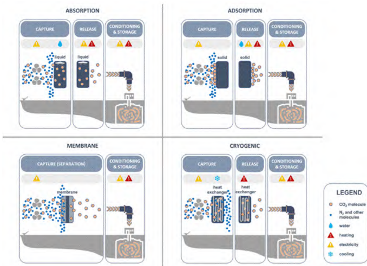
Figure 7: Roadmap for achieving scalable, safe, and low-cost direct air carbon capture and storage - Energy & Environmental Science - Royal Society of Chemistry
